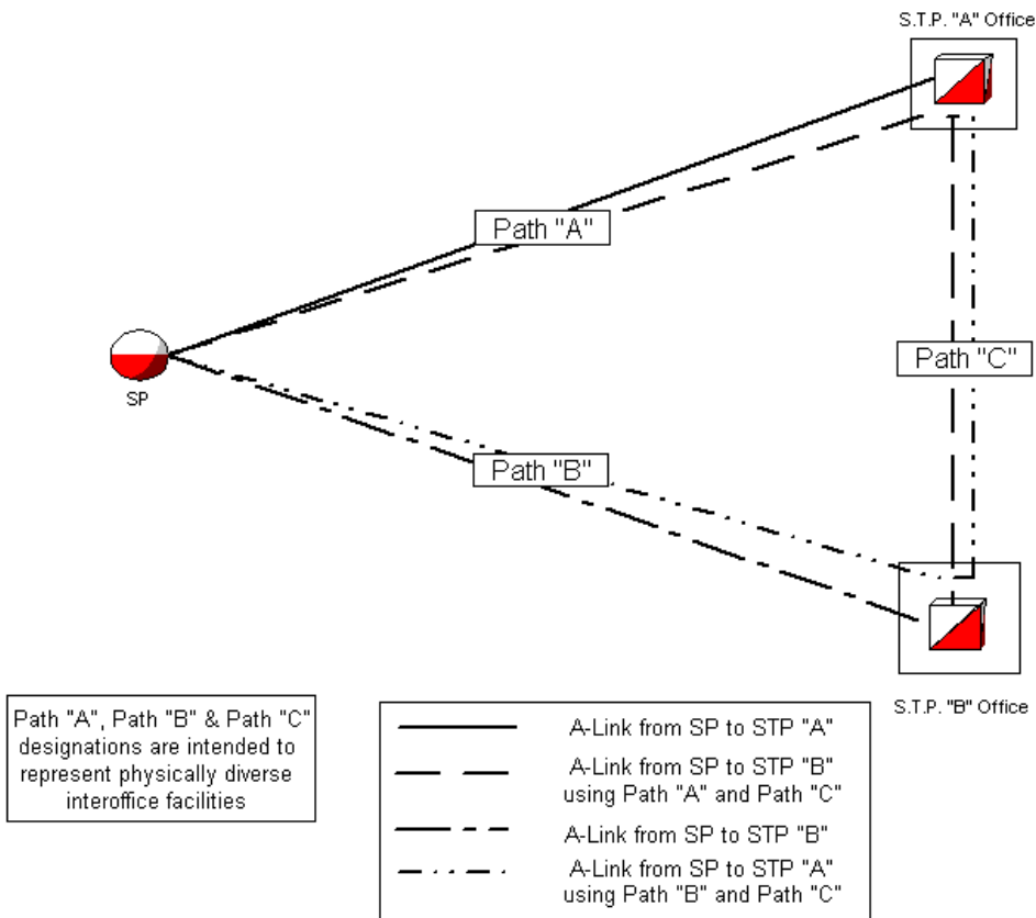
Figure 3: A-Link Crossover
