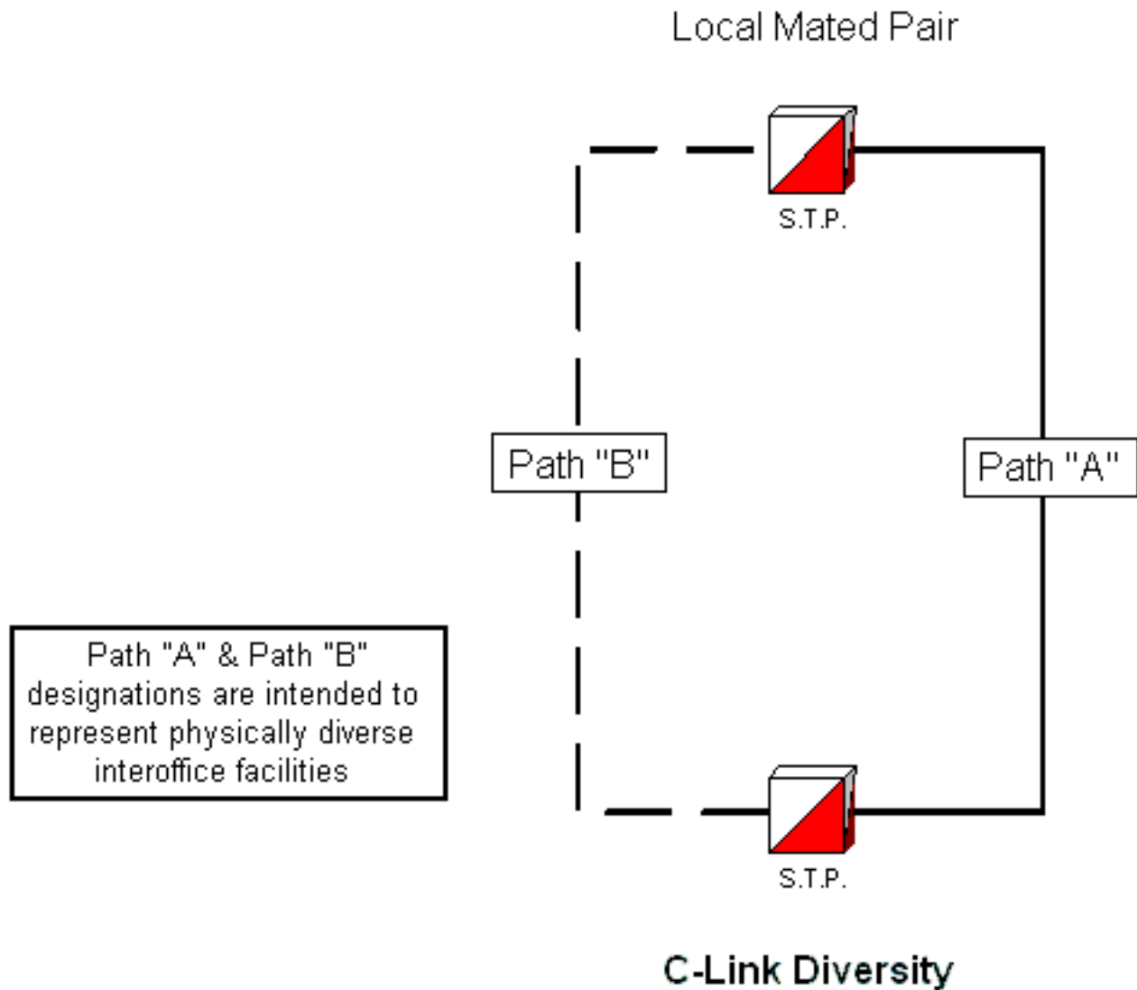
Figure 5: C-Link
