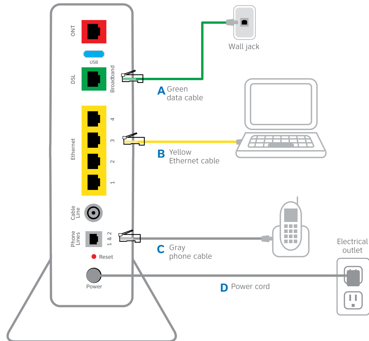
Wi-Fi Gateway
